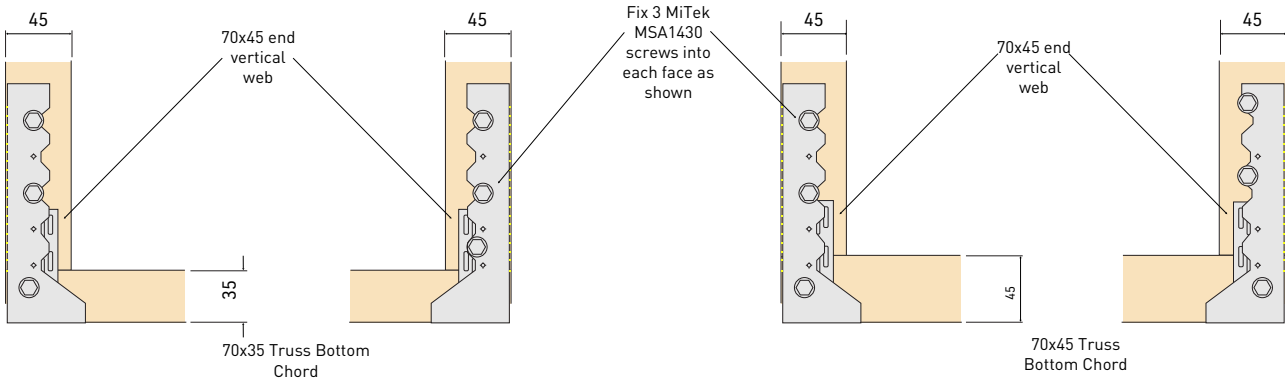
(i) Fixing Details for Joist Hanger JH70160
