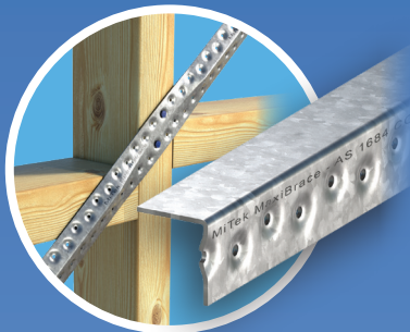
BRACING
