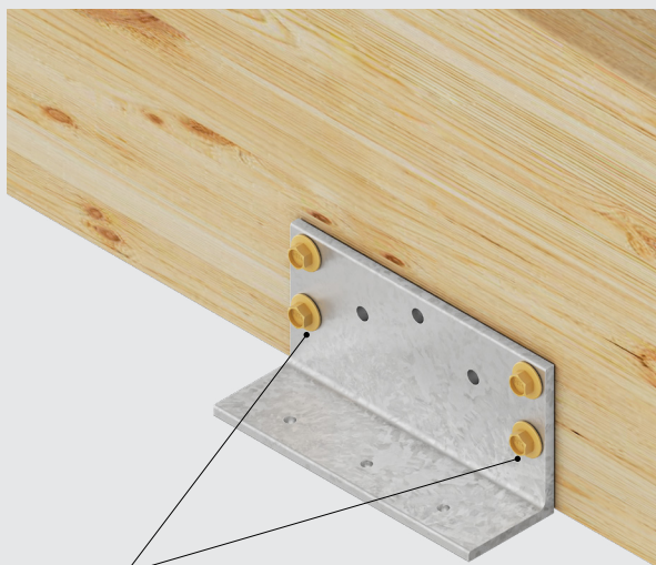
Fixing with 4 MiTek screws
