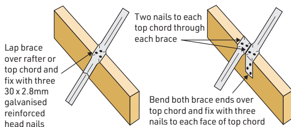
TYPICAL SPLICE DETAIL (OVERLAP SPLICE)
