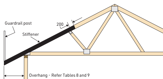
b) Truncated truss
