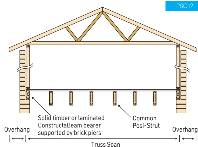
End wall - Single Storey EL = 2 \times \text{Overhang} + \text{Truss Span}
