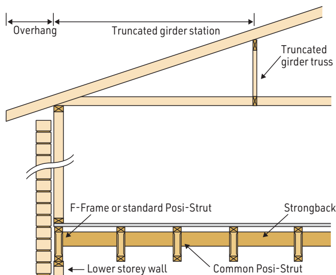
End wall - Building with Hip End Upper Storey of 2 Storey EL = \text{Truncated Girder Truss Station} + 2 \times \text{Overhang}
