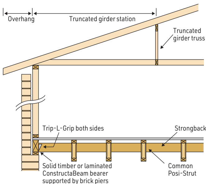
End wall - Building with Hip End Single Storey EL = \text{Truncated Girder Truss Station} + 2 \times \text{Overhang}
